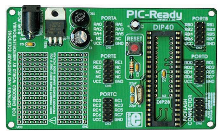
Figure 6: PIC-Ready development board
