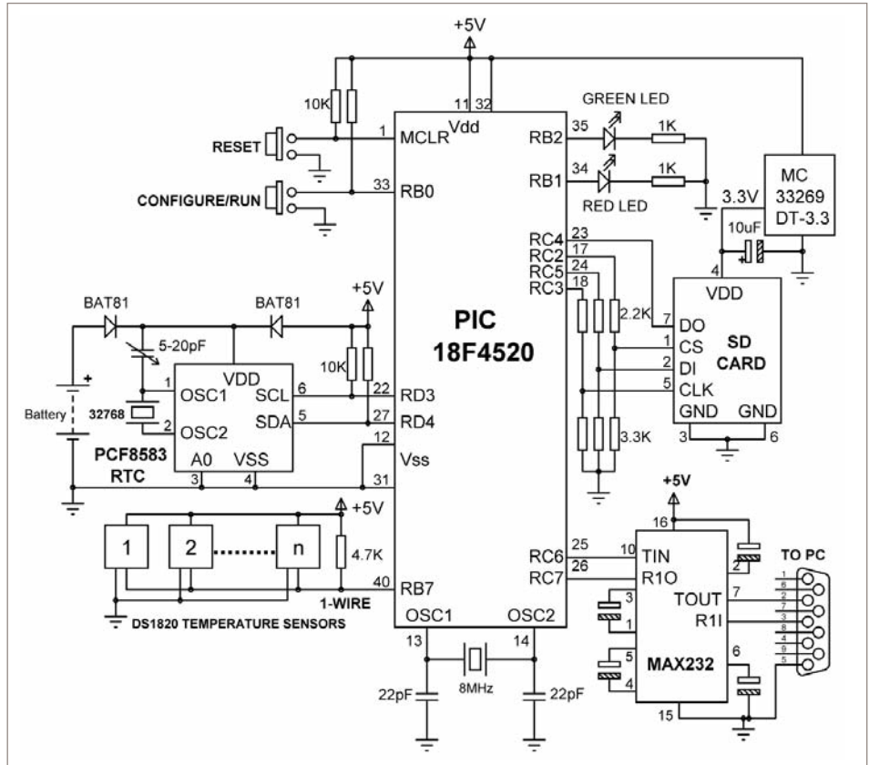
Figure 3: Circuit diagram of the temperature data logger device
