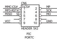
MP3's SDI interface
