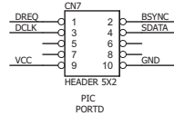
MP3's SDI interface
