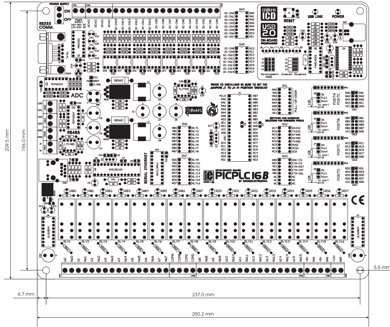
PIC-PLC16B Dimensions v100
