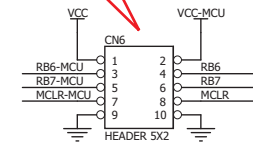
PICFlash CONNECTOR
