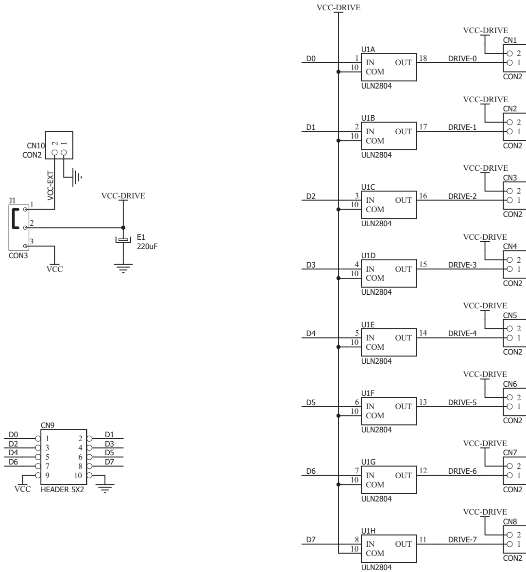
mikroDRIVE Schematic v100
