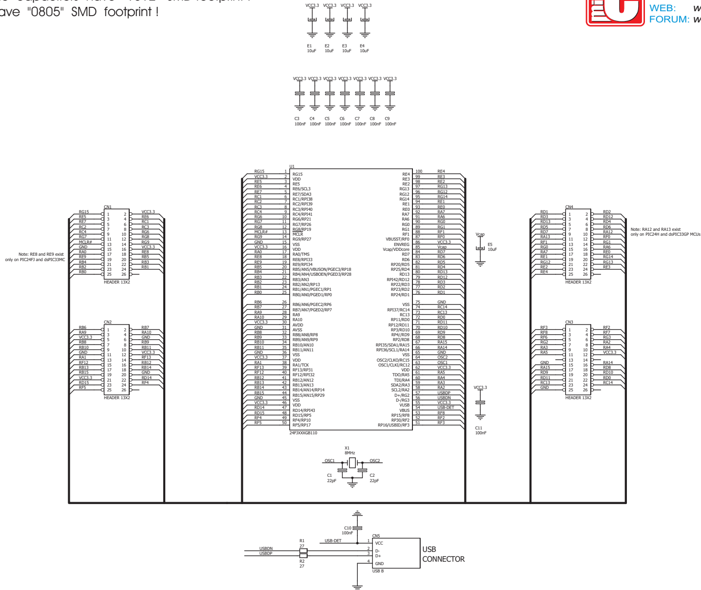
2433MCUcard16 Schematic v102
