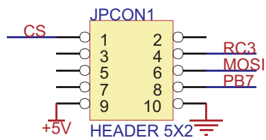
IDC10 connector
