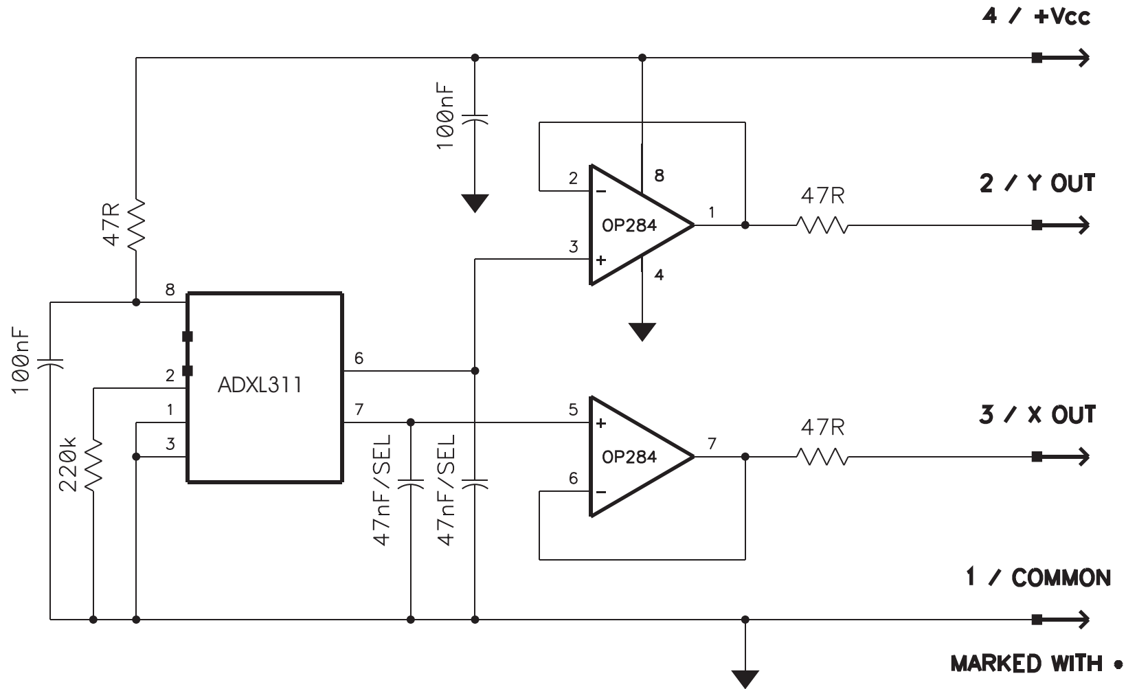
Acceleration Board Schematic
