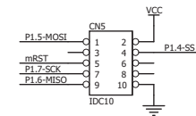
8051prog CONNECTOR
